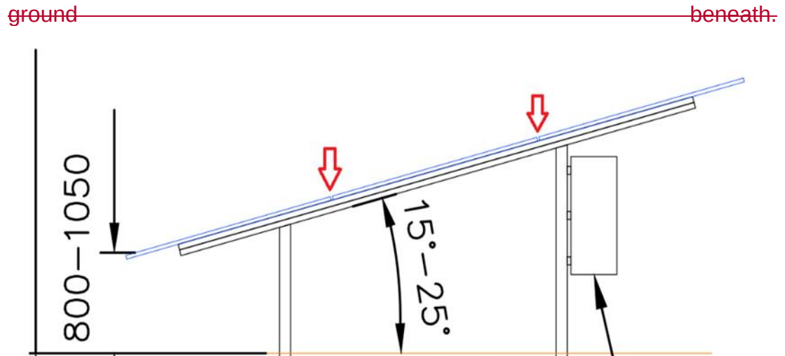
Figure 6. Typical Solar Array
